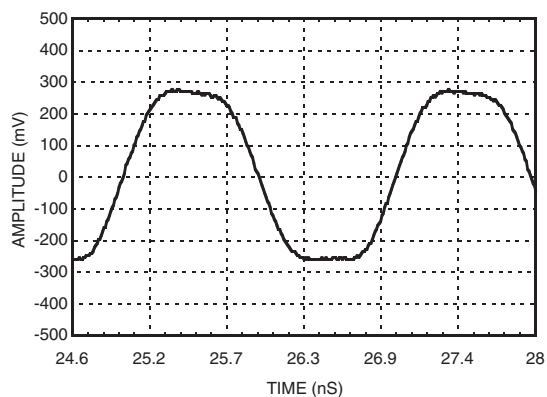
Output Voltage Waveform, P_{in} = 0 \text{ dBm} , F_{out} = 500 \text{ MHz} , T = 25^\circ\text{C}
