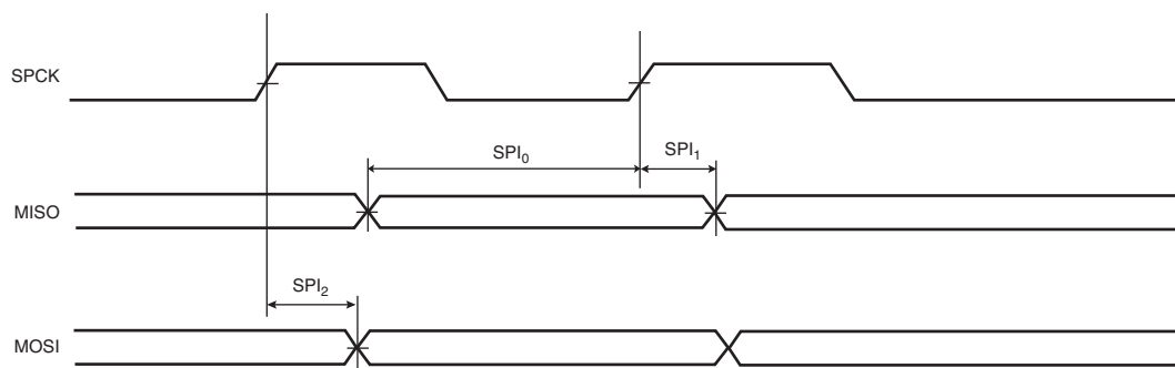
Figure 39-7. SPI Master mode with (CPOL=0 and NCPHA=1) or (CPOL=1 and NCPHA=0)
