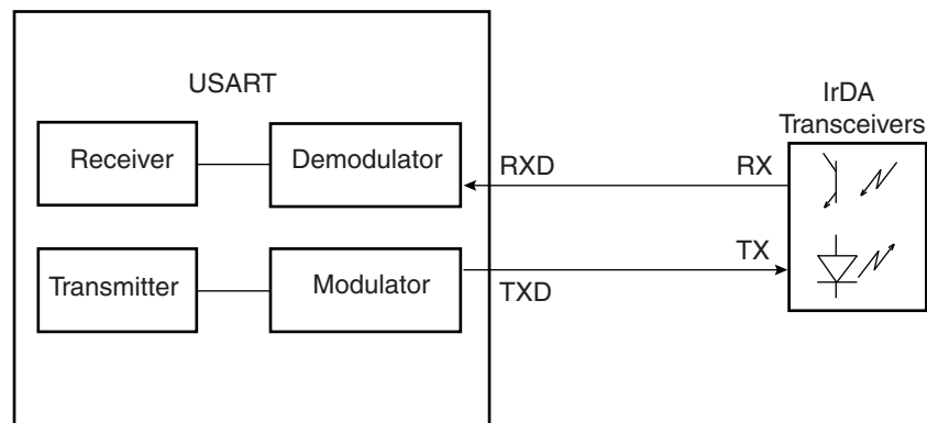
Figure 32-23. Connection to IrDA Transceivers
