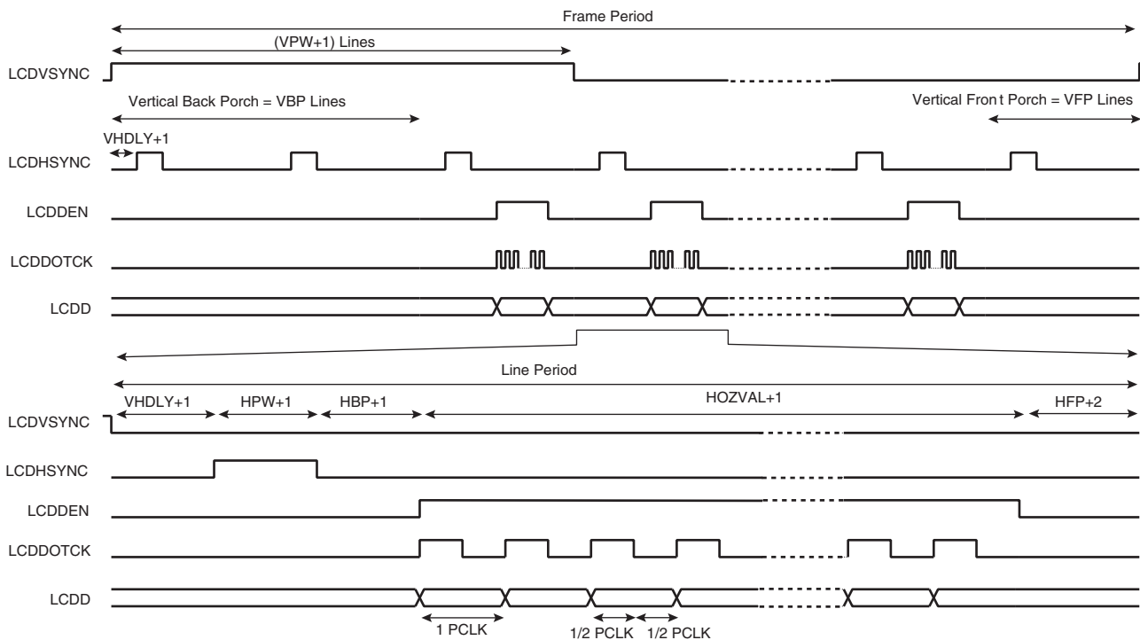
Figure 38-4. TFT Panel Timing, CLKMOD = 0, VPW = 2, VBP = 2, VFP = 1
