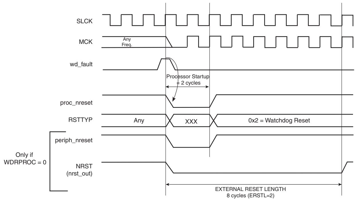
Figure 14-8. Watchdog Reset
