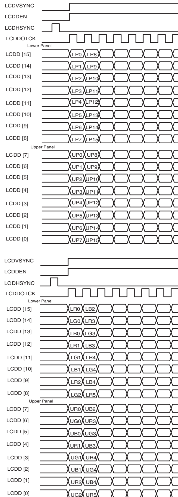
Figure 38-10. Dual Scan Monochrome and Color 16-bit Panel Timing (First Line Expanded View)
