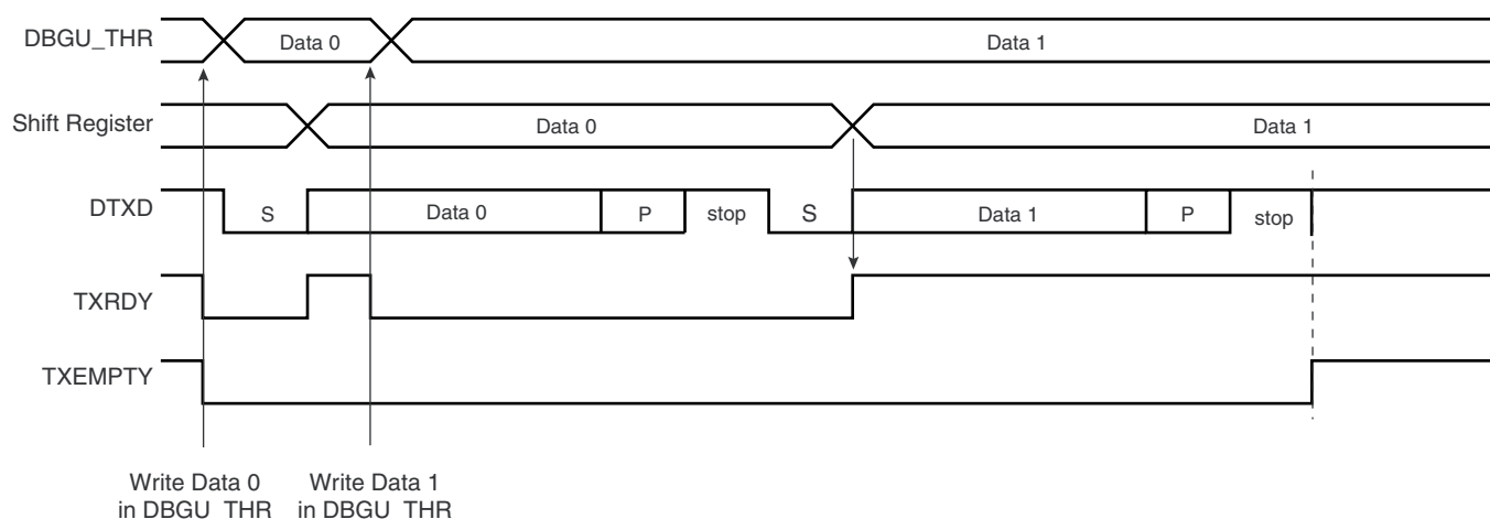
Figure 28-11. Transmitter Control
