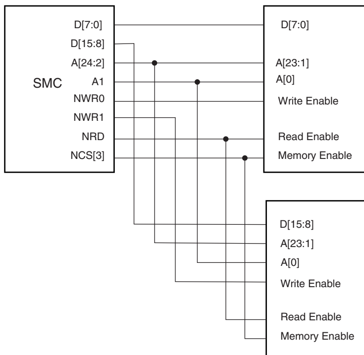
Figure 21-6. Connection of 2 x 8-bit Devices on a 16-bit Bus: Byte Write Option
