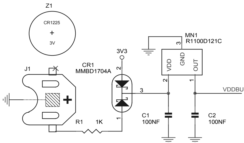
Figure 42-1. Schematic
