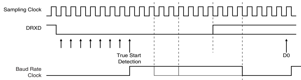
Figure 28-4. Start Bit Detection
