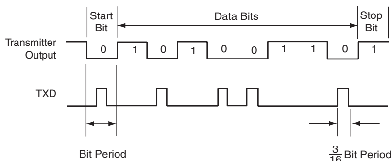
Figure 32-24. IrDA Modulation
