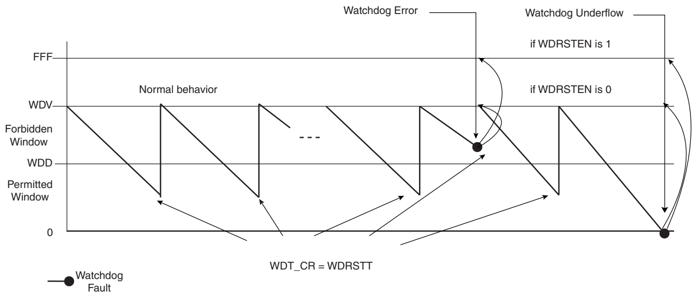
Figure 26-2. Watchdog Behavior
