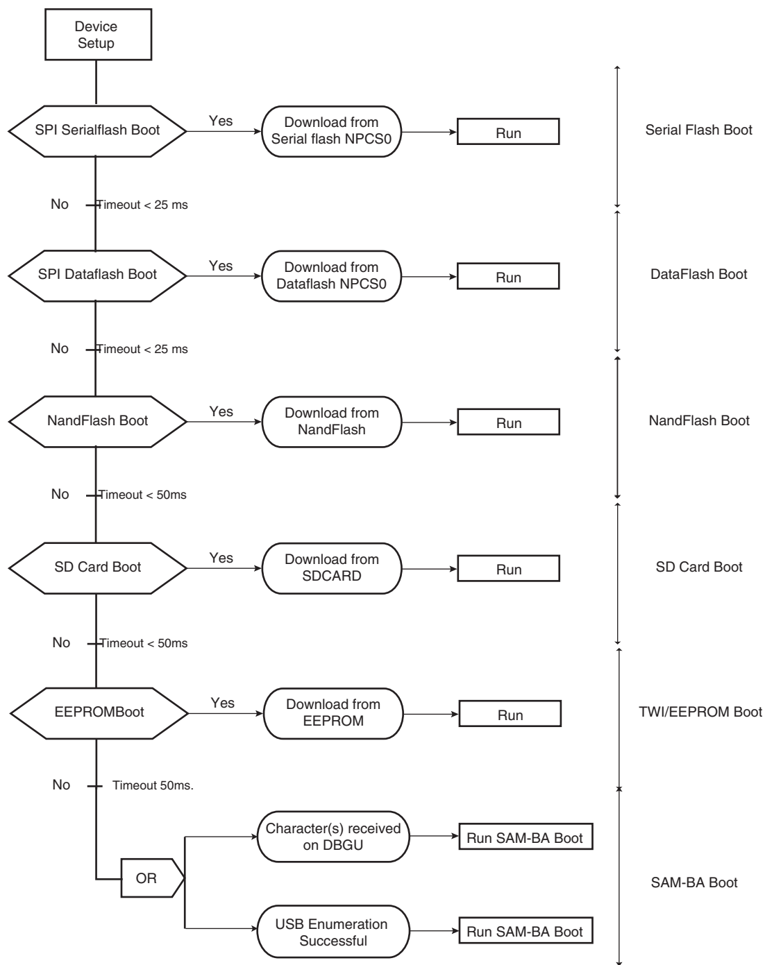
Figure 13-1. Boot Program Algorithm Flow Diagram
