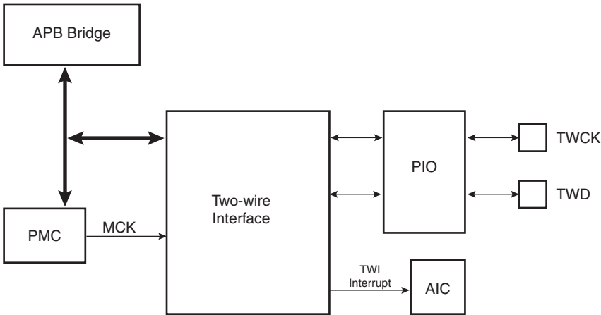
Figure 31-1. Block Diagram
