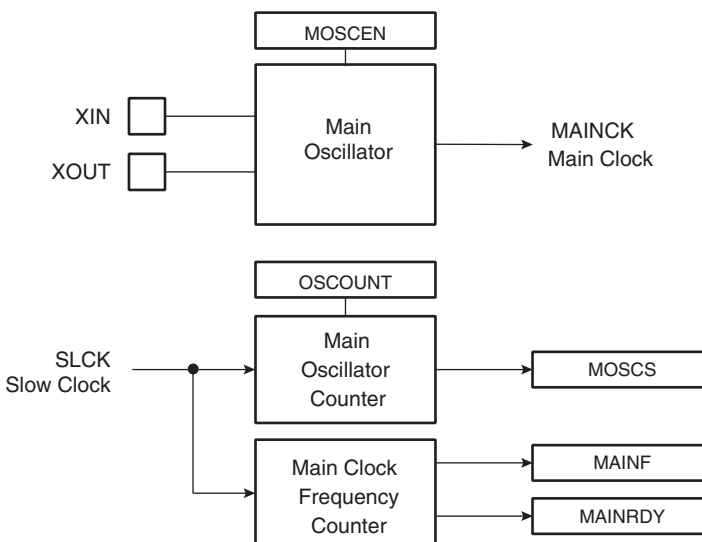
Figure 24-2. Main Oscillator Block Diagram
