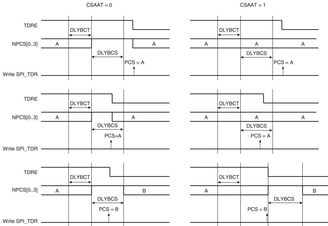
Figure 30-8. Peripheral Deselection
