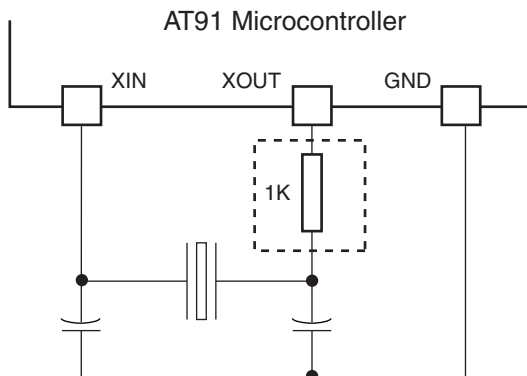
Figure 24-3. Typical Crystal Connection
