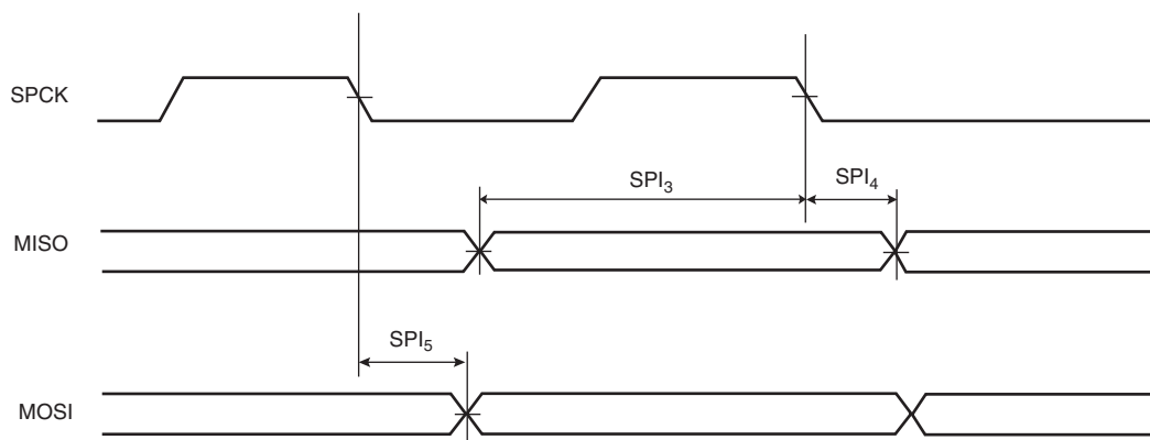
Figure 39-8. SPI Master mode with (CPOL = NCPHA = 0) or (CPOL= NCPHA= 1)
