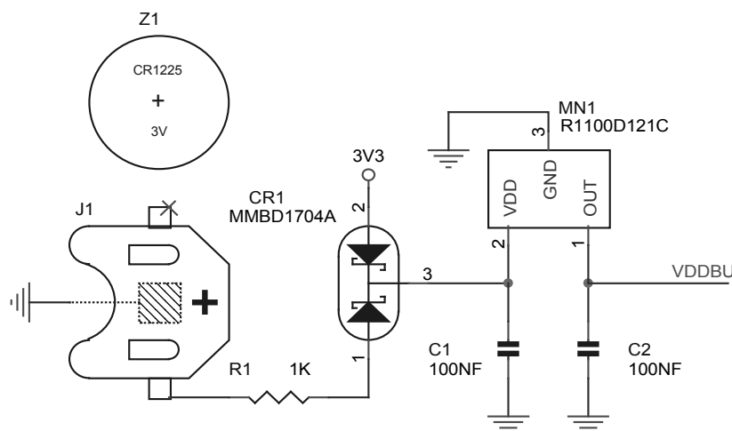
Figure 42-2. Schematic
