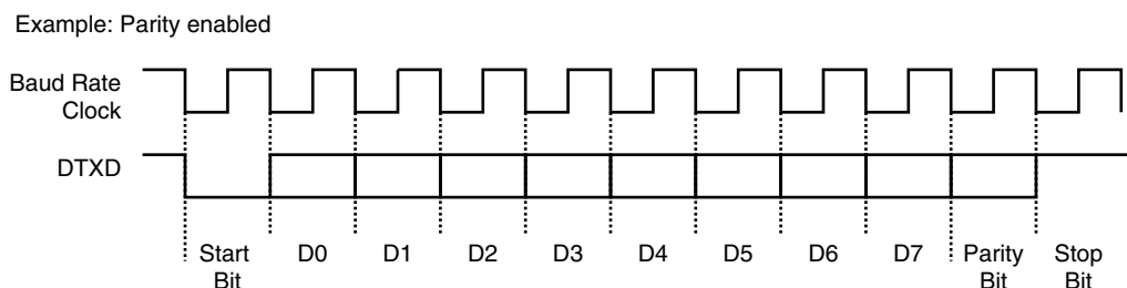
Figure 28-10. Character Transmission
