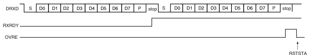
Figure 28-7. Receiver Overrun
