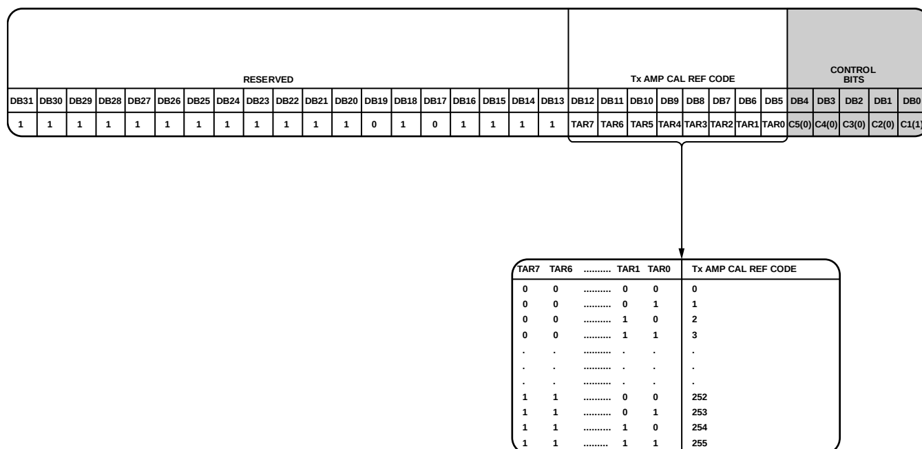
Figure 20. Register 1 (R1)
