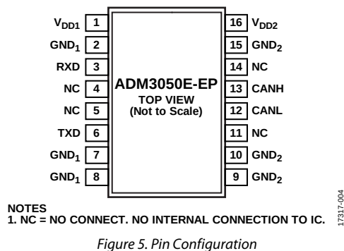
Figure 5. Pin Configuration
