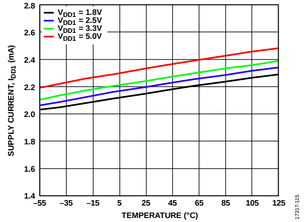
Figure 15. Supply Current ( I_{\text{DD1}} ) vs. Temperature
