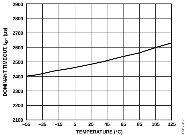
Figure 17. Dominant Timeout ( t_{\text{DT}} ) vs. Temperature
