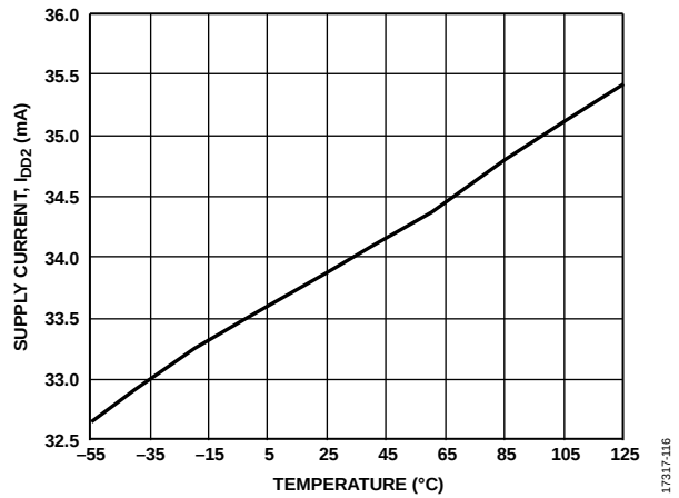
Figure 16. Supply Current ( I_{\text{DD2}} ) vs. Temperature
