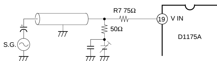
High frequency input measurement circuit
