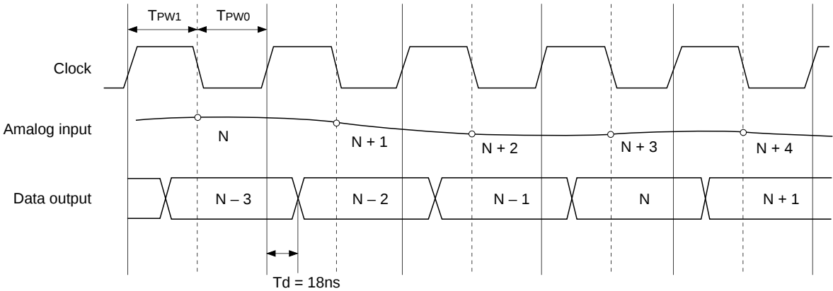
Timing Chart 1
