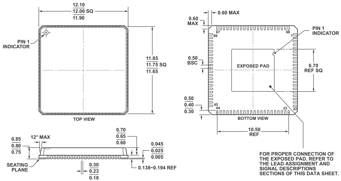
Figure 94. 88-Lead Lead Frame Chip Scale Package [LFCSQ_VQ] 1
