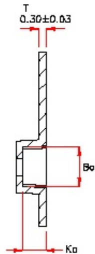
SECTION Y-Y
