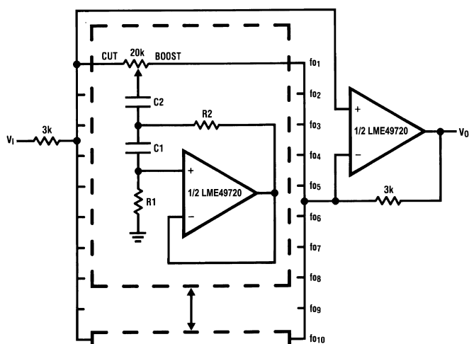
Figure 126. RIAA Preamp
