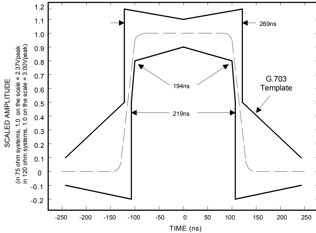
Figure 7-4. E1 Transmit Pulse Template
