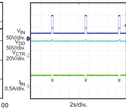
100V/0.4s Continuous Pulse V_{IN} = 24V , V_{OUT} = 5V , I_{OUT} = 2A
