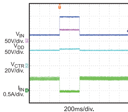
100V/0.4s Single Pulse V_{IN} = 24V , V_{OUT} = 5V , I_{OUT} = 2A
