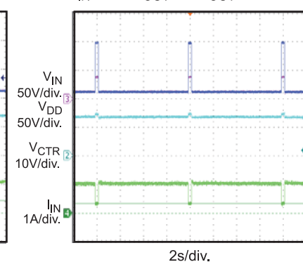
100V/0.3s Continuous Pulse V_{IN} = 12V , V_{OUT} = 5V , I_{OUT} = 2A
