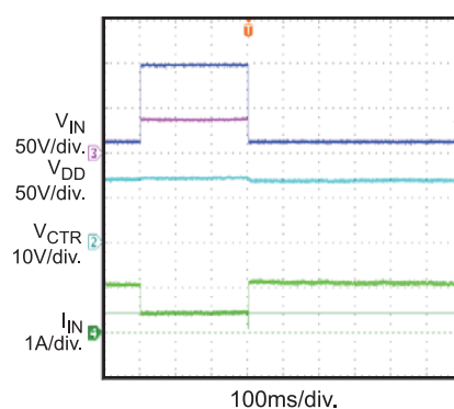
100V/0.3s Single Pulse V_{IN} = 12V , V_{OUT} = 5V , I_{OUT} = 2A
