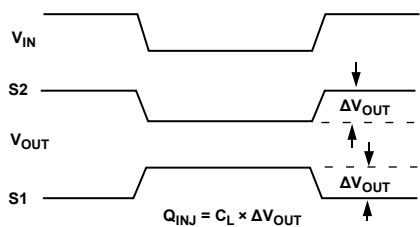
Figure 21. Charge Injection
