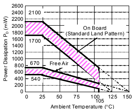
Power Dissipation
