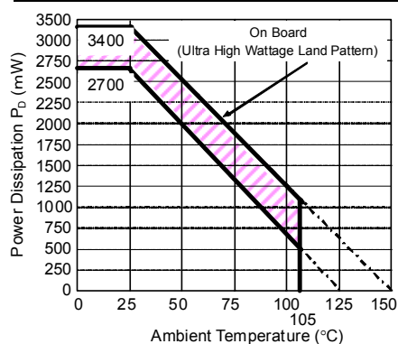
Power Dissipation
