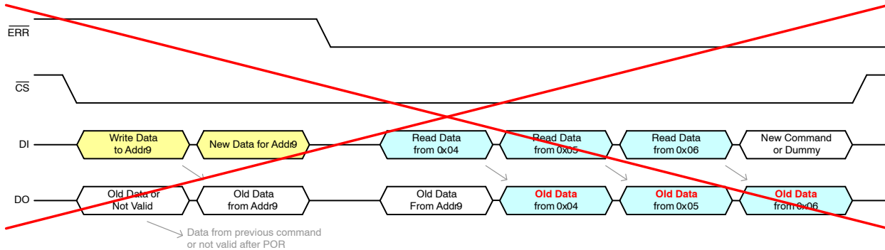
Figure 33. Bad Example of Error Read Out
