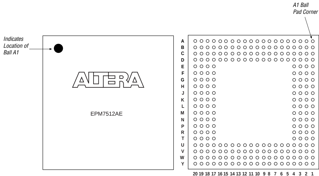
Package outline not drawn to scale.
