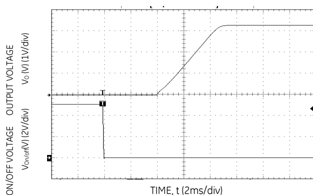
Figure 15. Typical Start-Up Using Remote On/Off with Low-ESR external capacitors (7x150uF Polymer) ( V_{in} = 5.0\text{Vdc} , V_o = 3.3\text{Vdc} , I_o = 3\text{A} , C_o = 1050\text{ }\mu\text{F} ).
