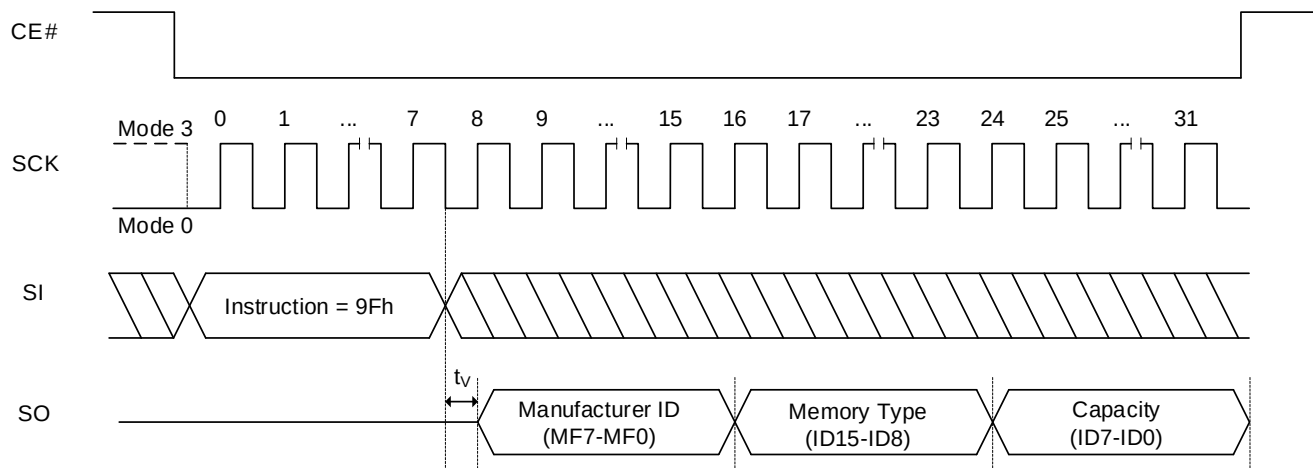
Figure 8.50 RDJID (Read JEDEC ID) Sequence in SPI mode
