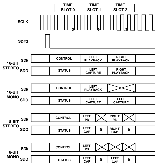
Figure 31. Serial Data Format, 2-Wire System (TSSEL = 1)
