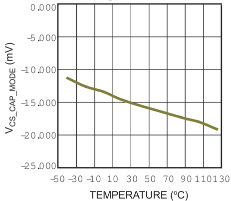
CS Capacitive Mode Detection Threshold vs. Temperature
