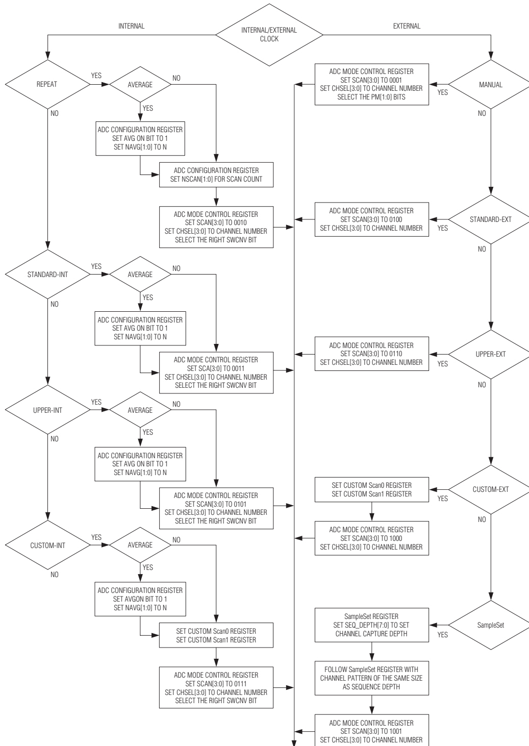
Figure 12. ADC Mode Select Programming Sequence
