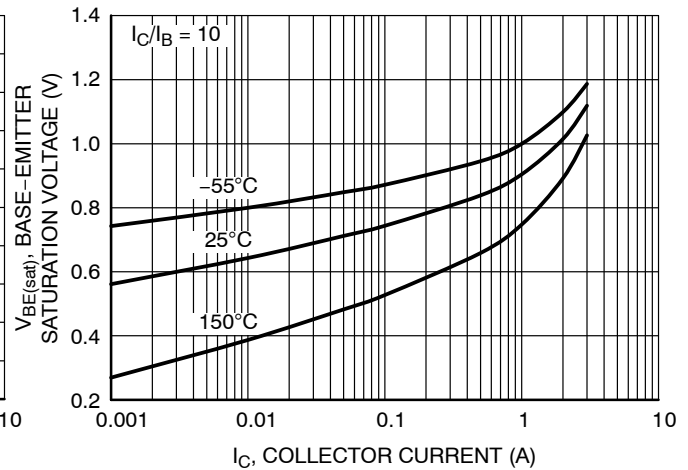
Figure 18. Base-Emitter Saturation Voltage
