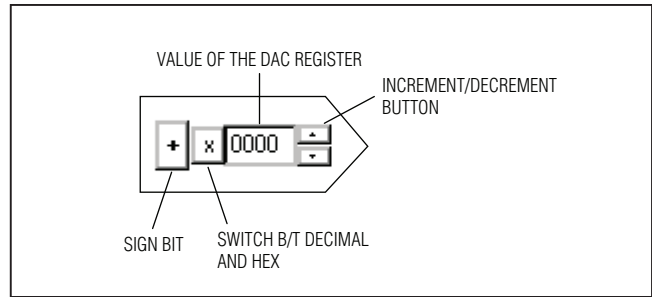
Figure 3. Register Controls
