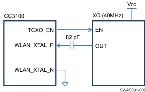
Figure 4-11. External TCXO Input
