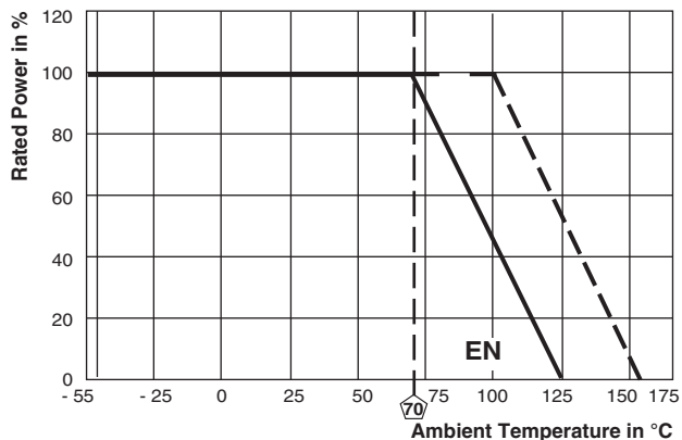
Derating
