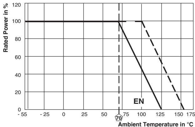
Derating
