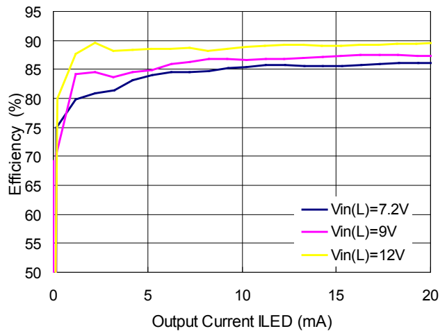
6LED, V_{IN(IC)}=3.6V
