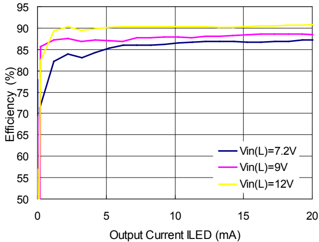
5LED, V_{IN(IC)}=3.6V
