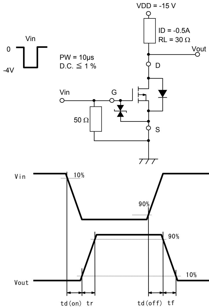
*2 Measurement circuit for Turn-on Delay Time/Rise Time/Turn-off Delay Time/Fall Time
