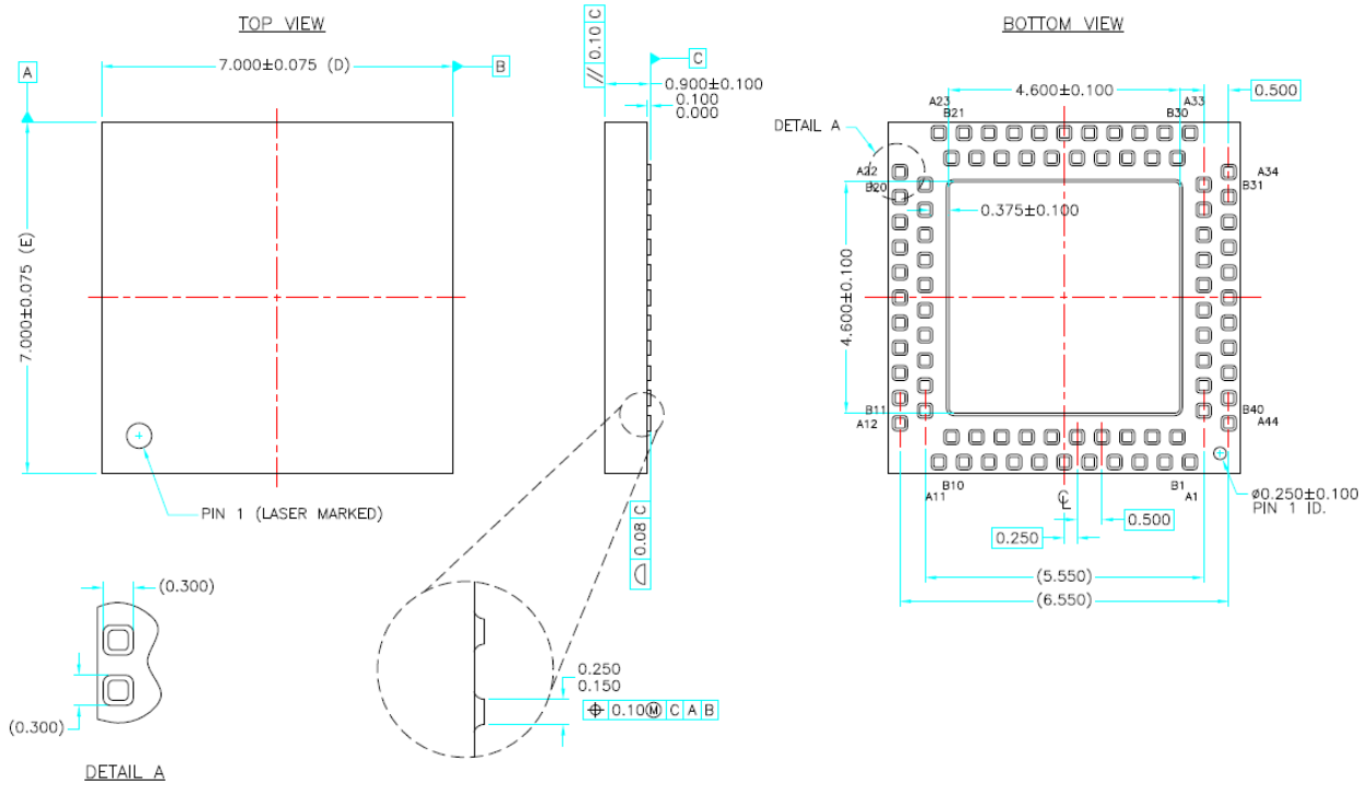
Figure 9 : Package dimensions
