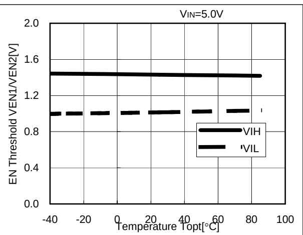
14) Enable Input Voltage vs. Temperature
