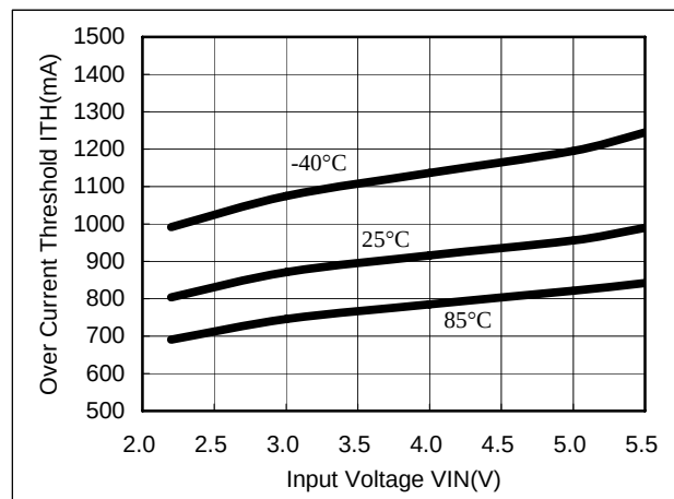
13) Over Current Threshold vs. Input Voltage
