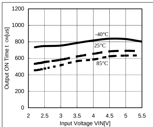
7) Output On Time vs. Input Voltage
