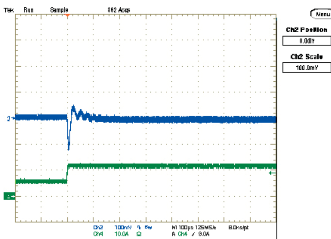
Step Load Transient Response (Vin=12V, Vout=3.3V, Cload=188μF, Iout=6A to 12A) Trace 2=Vout, 100 mV/div, Trace 4=Iout, 10A/div.
