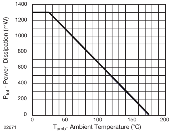
22671 Fig. 1 - Admissible Power Dissipation vs. Ambient Temperature P_{tot} = f(T_{amb})
