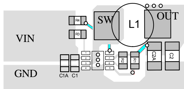
Figure 3: Recommended PCB Layout
