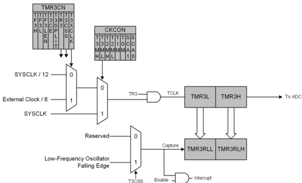
Figure 25.10. Timer 3 Capture Mode (T3SPLIT = 0)
