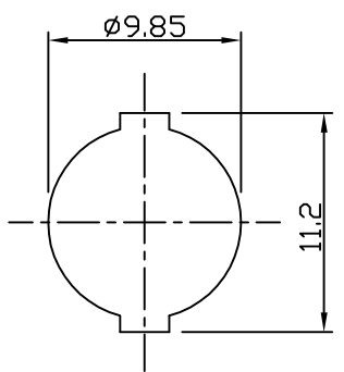
PANEL CUTOUT
