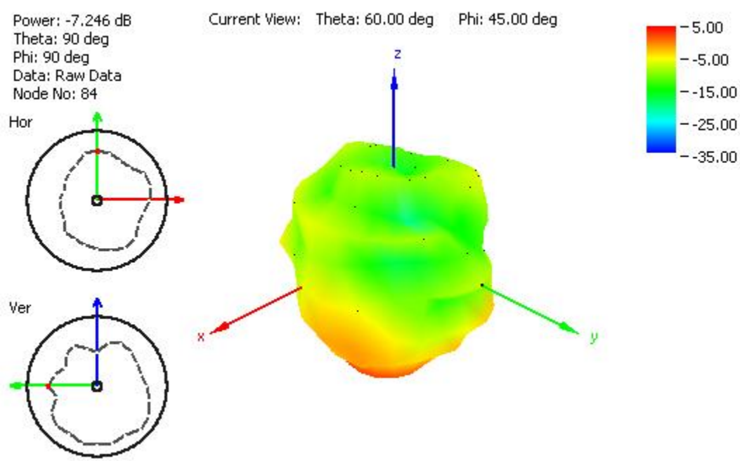
Figure 17. Radiation pattern at 915 MHz, Figure 1 as reference (dB), with 2 m RG174 cable and 30x30 cm metal plate.
