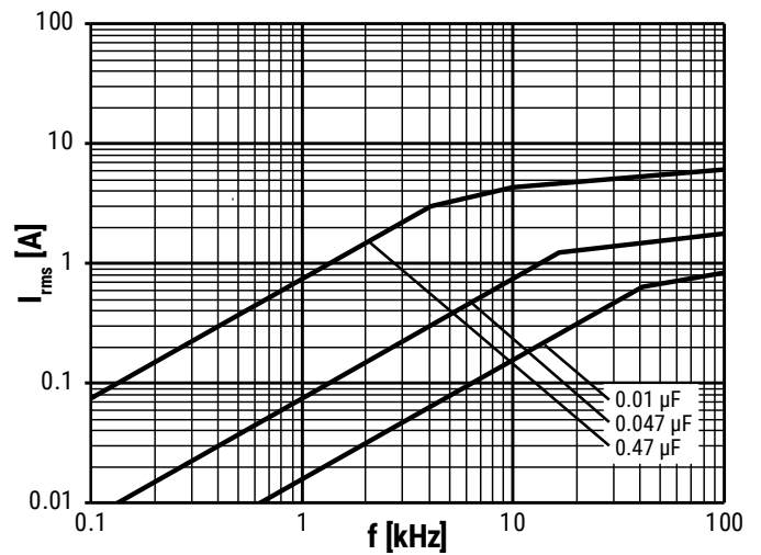
630 VDC/250 VAC
