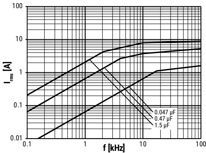
400 VDC/220 VAC
