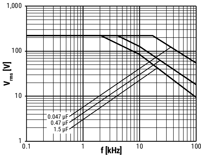
400 VDC/220 VAC
