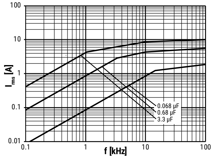
250 VDC/200 VAC
