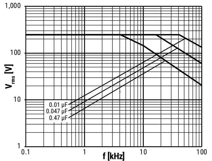
630 VDC/250 VAC
