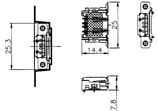
CONNECTOR DETAIL
