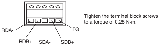
RS-422A/485 Connector
