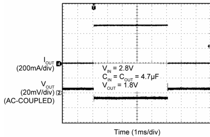
Load Transient
