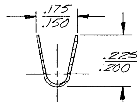
SECT. B-B
