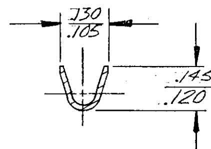
SECT. A-A
