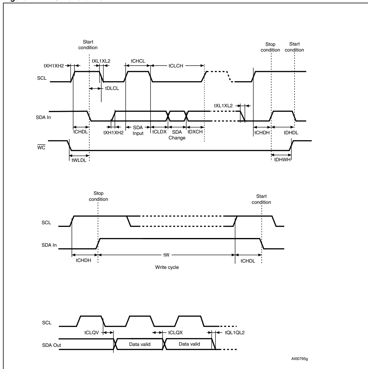
Figure 14. AC waveforms
