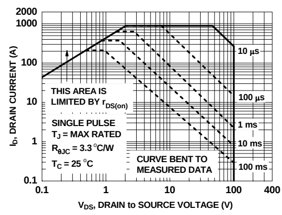
Figure 12. Forward Bias Safe Operating Area for FDPF2D3N10C
