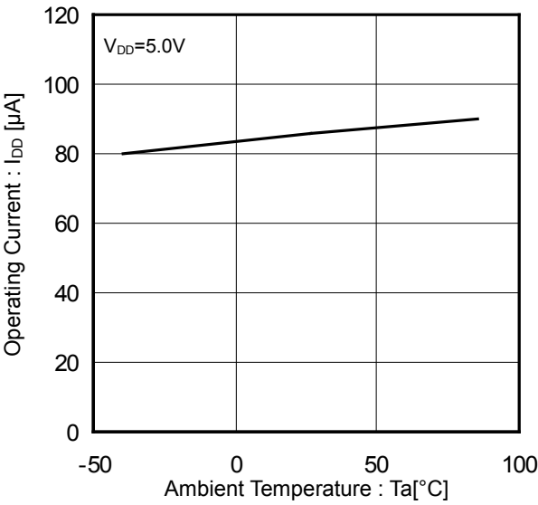
Figure 4. Operating Current vs Ambient Temperature (CTRL Enable)
