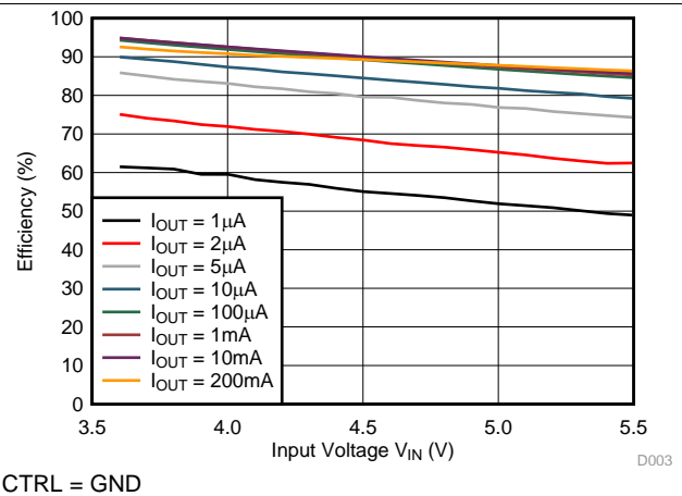
Figure 8. TPS82740A Efficiency V_{OUT} = 2.1V
