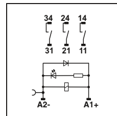
DC coils
