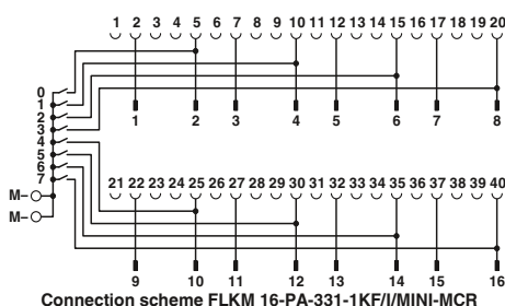
Connection scheme FLKM 16-PA-331-1KF/I/MINI-MCR
