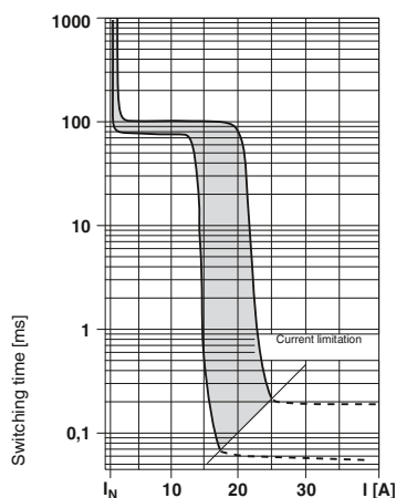
Time-current characteristic, 4 A version
