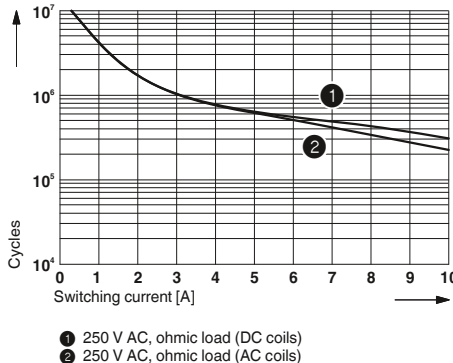
Electrical service life for PLC-RSP...UC/21HC/RW
