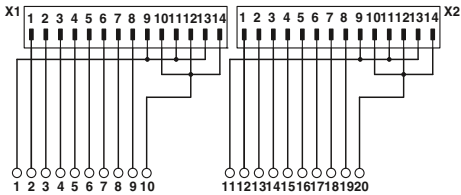
Connection scheme: VIP-2/.../2FLK14 (1-20) /S7
