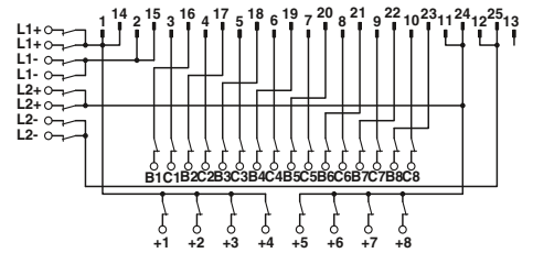
FLKM-D25 SUB/B/KDS3-MT/TU810/P connection scheme
