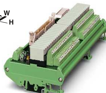
Output modules with 32 miniature relays, 1 N/O contact
