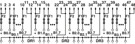
Connection scheme: FLKM 50/32M/SI/PLC
