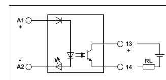
Figure 3: 2-conductor output
