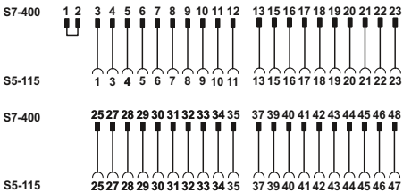
Connection scheme: FLKM S115/S400/SO155
