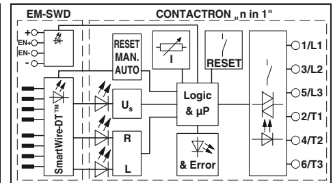
Reversing starter + emergency stop + motor protection + SmartWire-DT™ adapter, as a set 550 V AC/3 x 9 A
