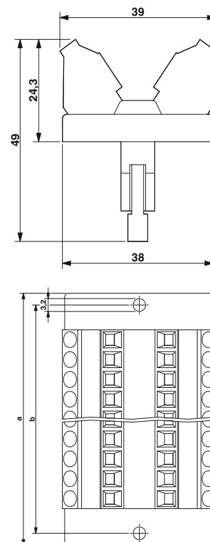
Dimensional drawing DFLK:
